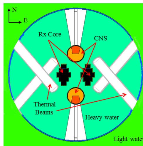
Fig. 1. Schematic of the reactor components.
